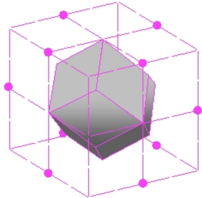
Brillouin Zone = Wigner-Seitz Cell for Reciprocal Lattice
